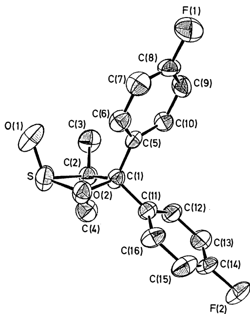
FIGURE The molecular structure of S(O)OC(Me)_2C(p-C_6H_4F)_2 showing the atomic numbering. Hydrogen atoms have been omitted
