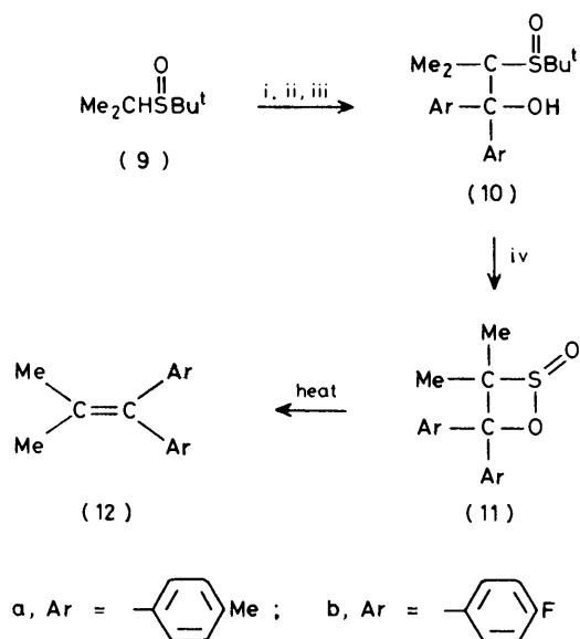
SCHEME 1 Reagents: (i) \text{Bu}^t\text{Li} ; (ii) \text{Ar}_2\text{C}=\text{O} ; (iii) \text{H}_2\text{O} ; (iv) \text{SO}_2/\text{Cl}_2
